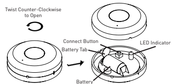
Figure 2 - Opening the Leak Sensor
